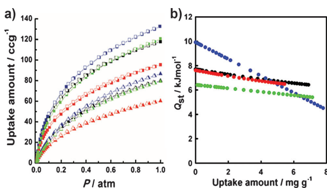
Figure 3. Gas-adsorption properties of SNU-200' (black), [K + ⊂SNU-200'·SCN - ] (navy), [NH 4 + ⊂SNU-200']·Cl - (green) and [MV 2+ ⊂SNU-200']·2Cl - (red) a) H 2 gas sorption isotherms at 77 K (square) and 87 K (triangle). Filled shape: adsorption; open shape: desorption. b) Isosteric heat ( Q st ) of H 2 adsorption.
